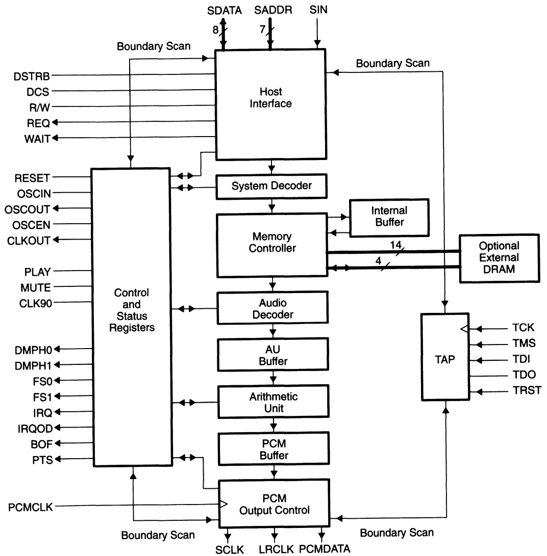
Figure 12–1. TMS320AV110 Block Diagram
