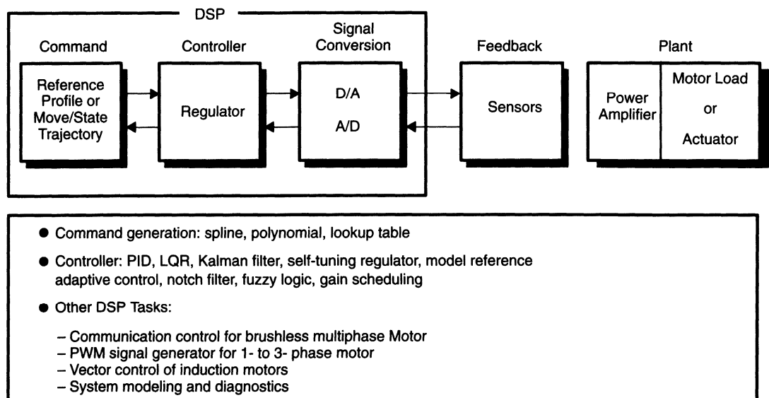
Figure 1–13. Digital Motor Control
