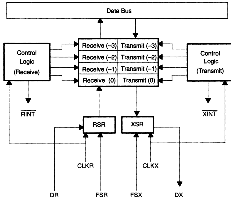
Figure 5-1. TMS320C2xx Synchronous Serial Port
