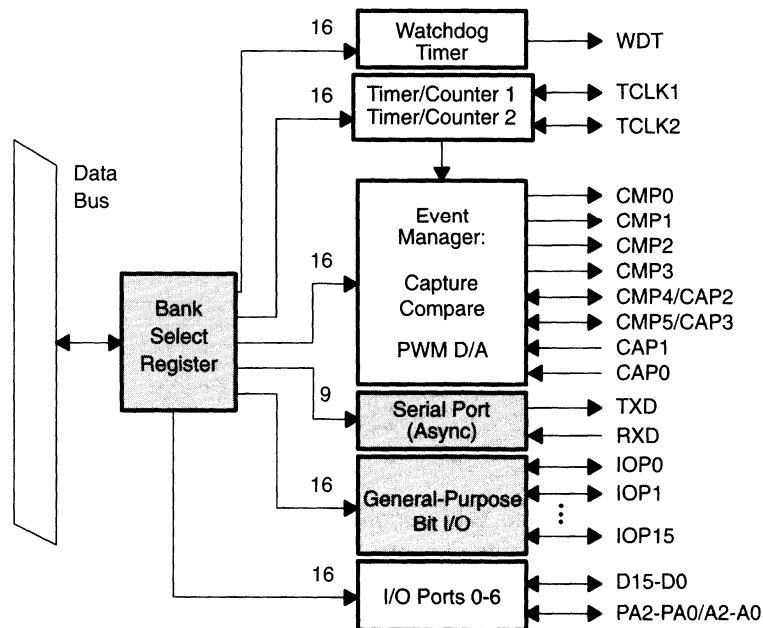
Figure 3–4. TMS320C14 Peripherals
