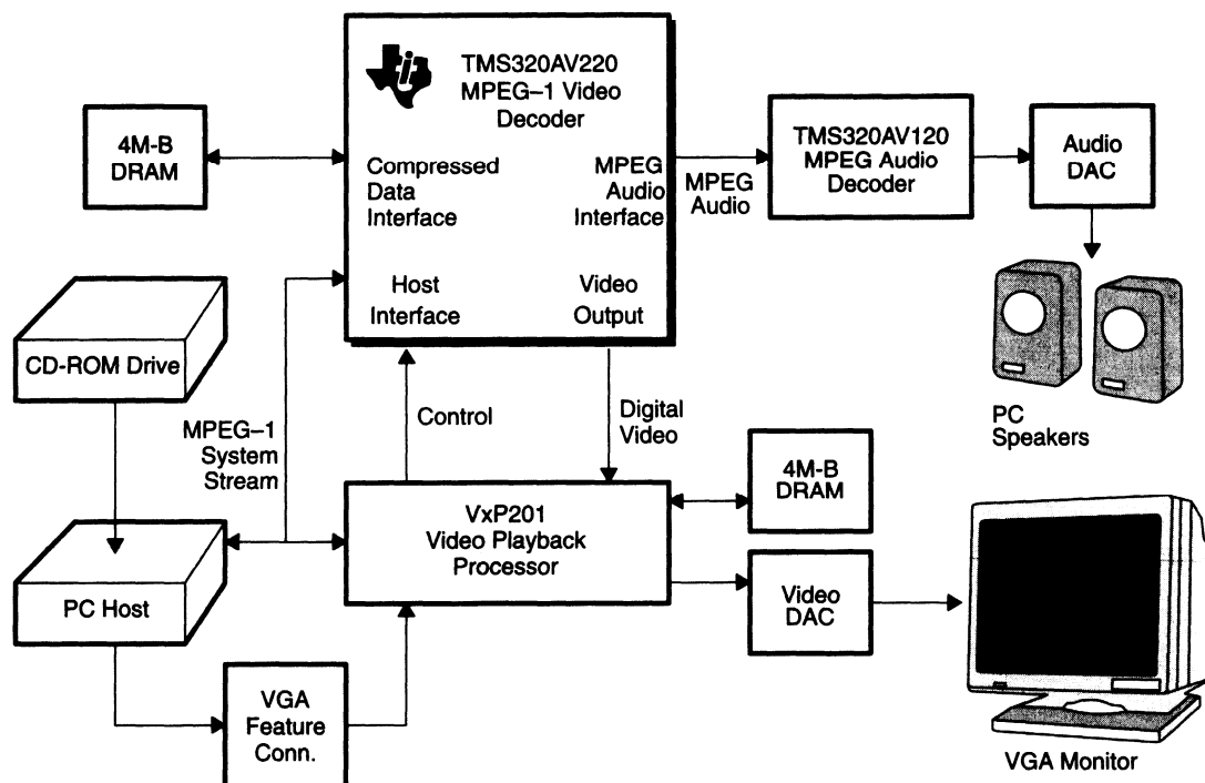
Figure 1-11. TI MPEG Solution
