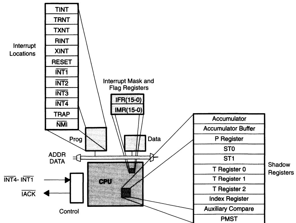
Figure 9–5. TMS320C5x Interrupts
