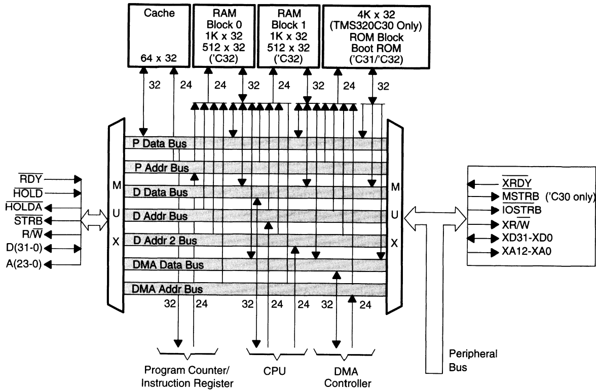
Figure 7-2. TMS320C3x Memory
