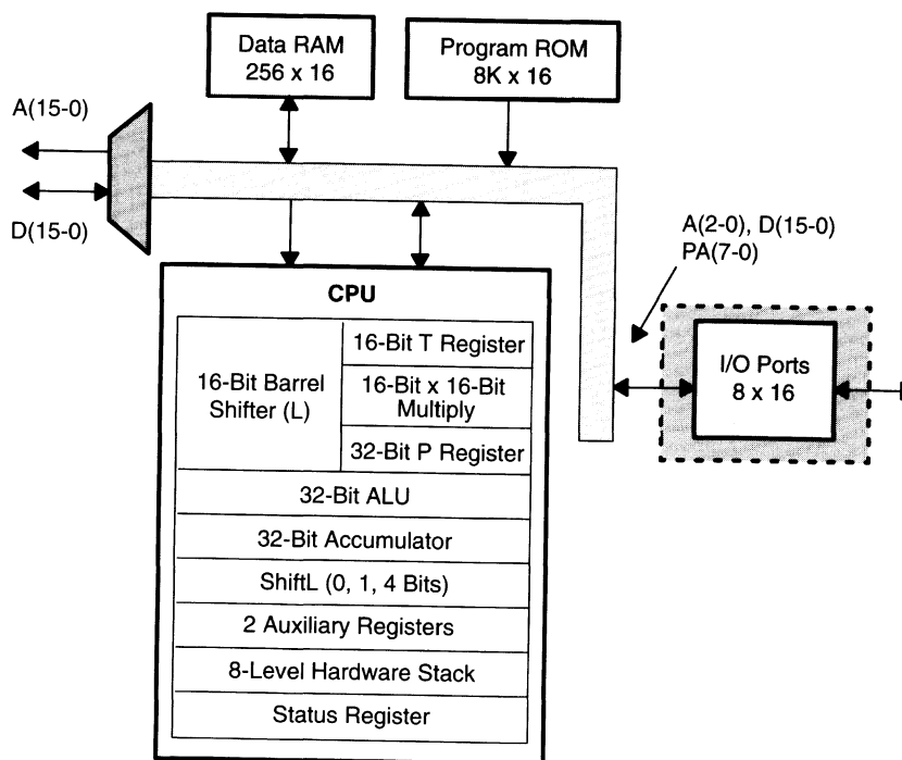
Figure 3–6. TMS320C16 Block Diagram
