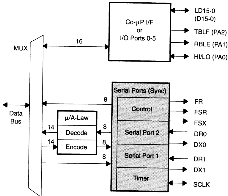
Figure 3–8. TMS320C17 Peripherals
