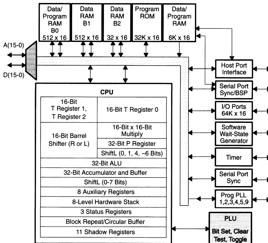
Figure 9–14. TMS320LC57 Block Diagram
