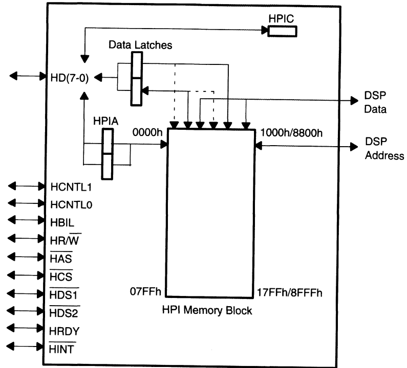
Figure 9-1. TMS320LC57/BC57S Host Port Interface
