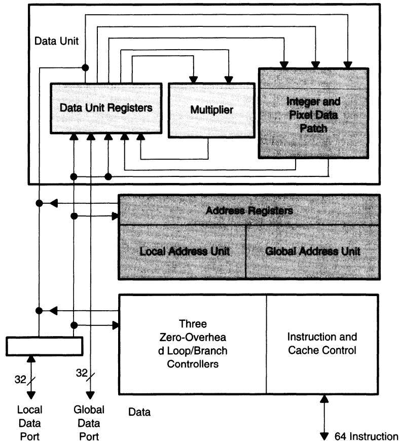
Figure 11–3. TMS320C8x Parallel Processing Advanced DSPs (PP)
