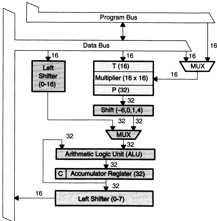
Figure 4–1. TMS320C2x Multiplier/ALU
