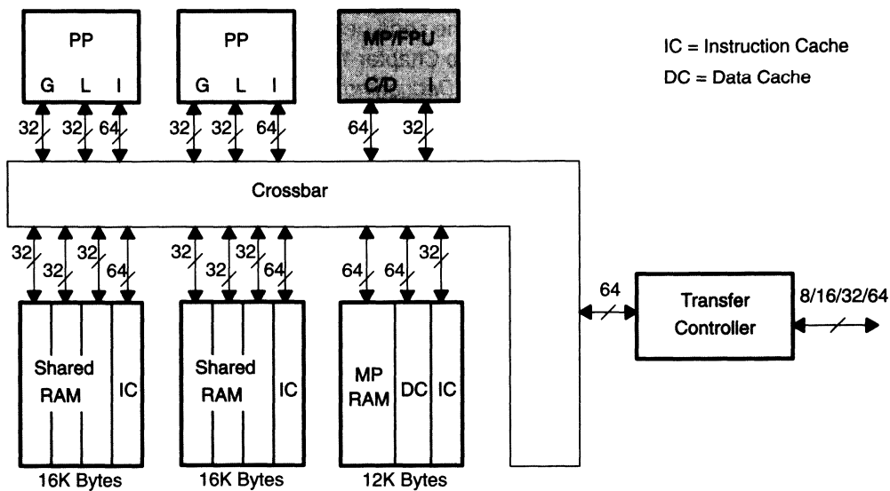
Figure 11–8. TMS320C82 Block Diagram
