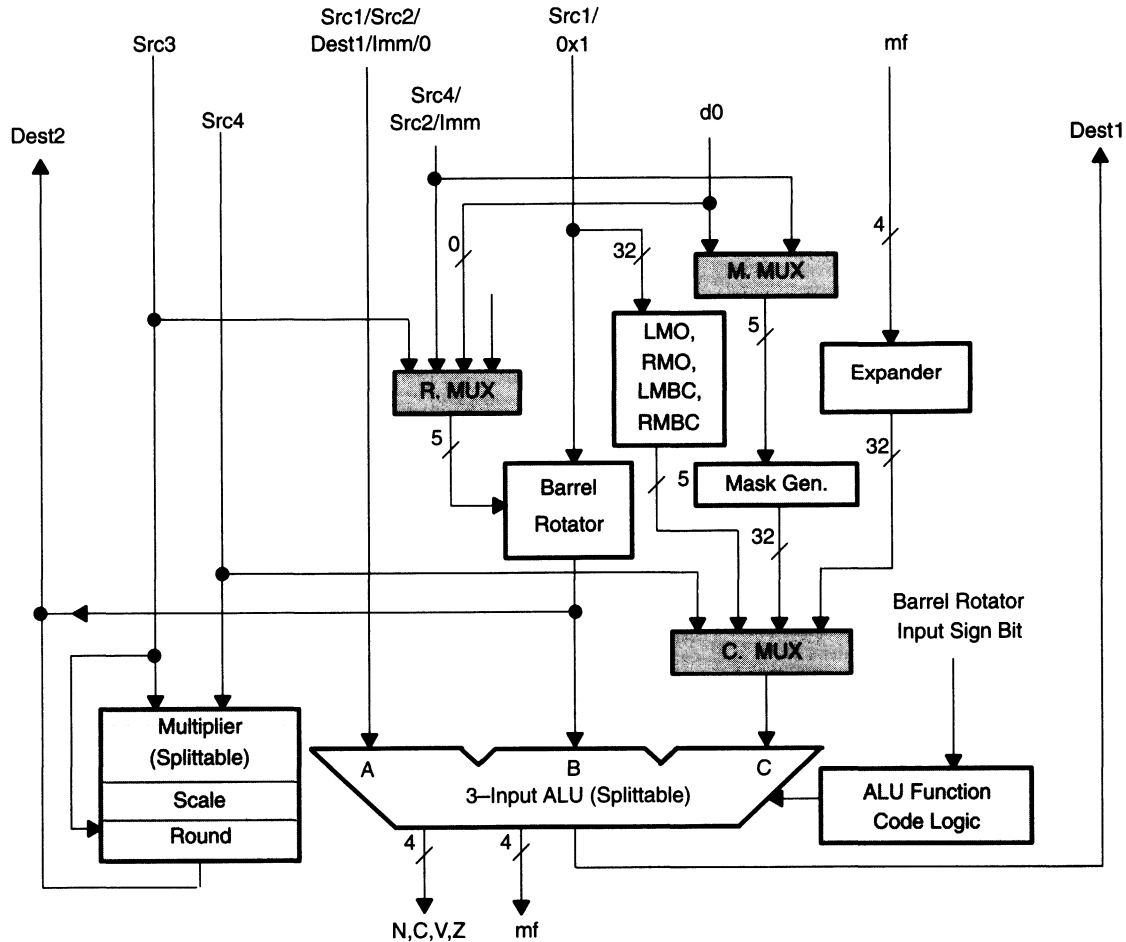
Figure 11–4. TMS320C8x PP Data Unit
