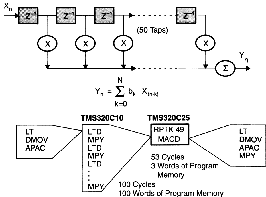
Figure 4–3. TMS320C25 Sum of Products Example
