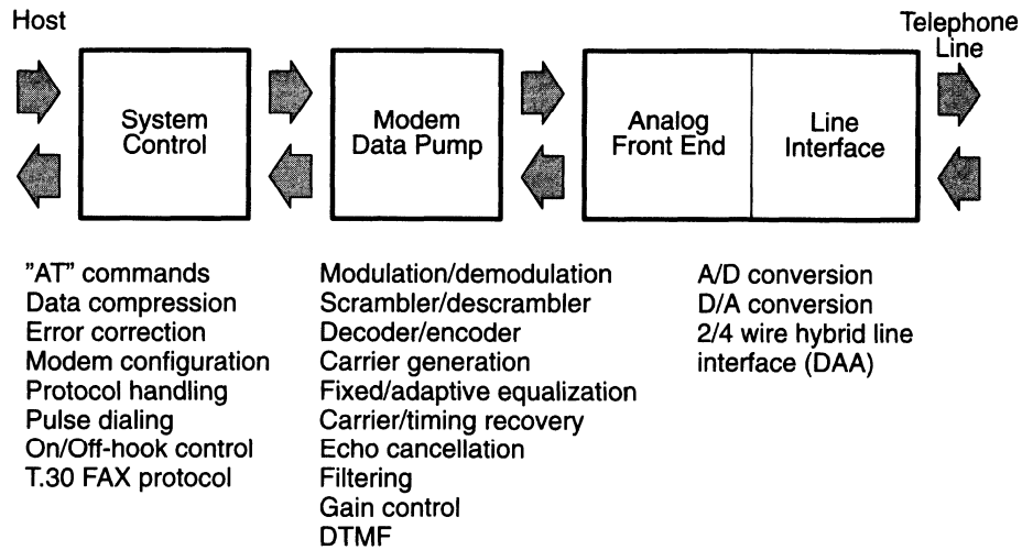
Figure 1–5. Modem Tasks
