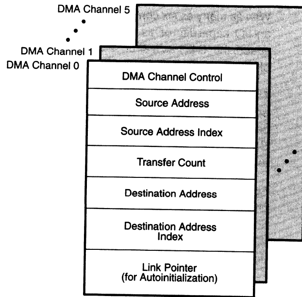
Figure 8-4. TMS320C4x DMA Coprocessor
